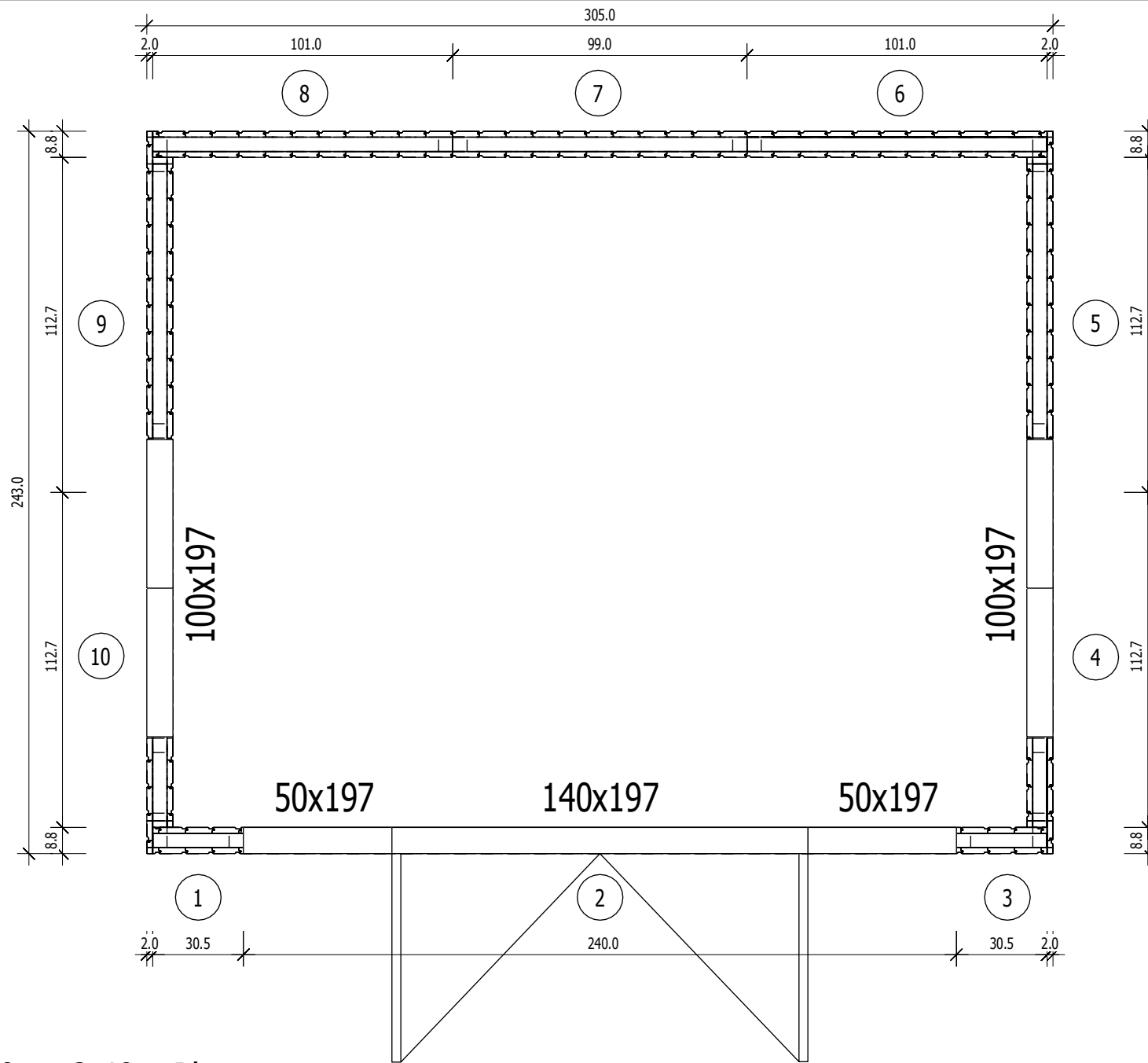
Lomond 3.00m x2.40m Plan
